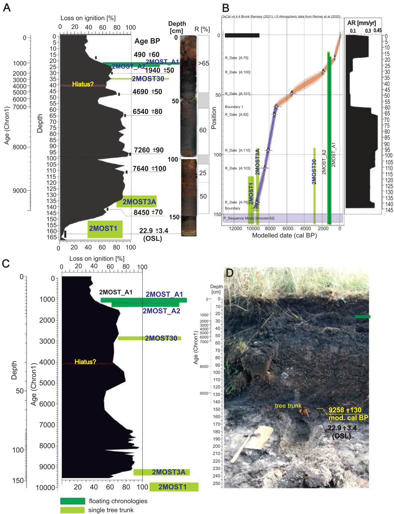
Fig. 4. Sedimentary sequence of the Mosty peatland
